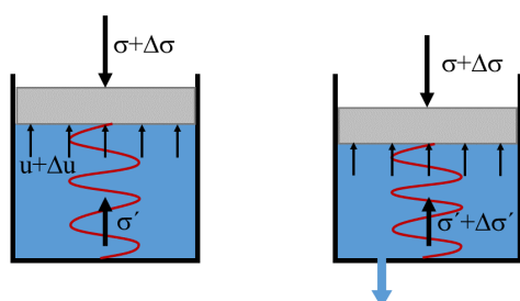
Figur 4: Komprimerings prinsipp (NGU, 2018)
