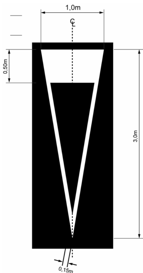
Figur 6.12: Skisse for vikesymbol
