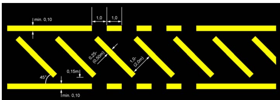
Figur 6.15: Skisse skravering
