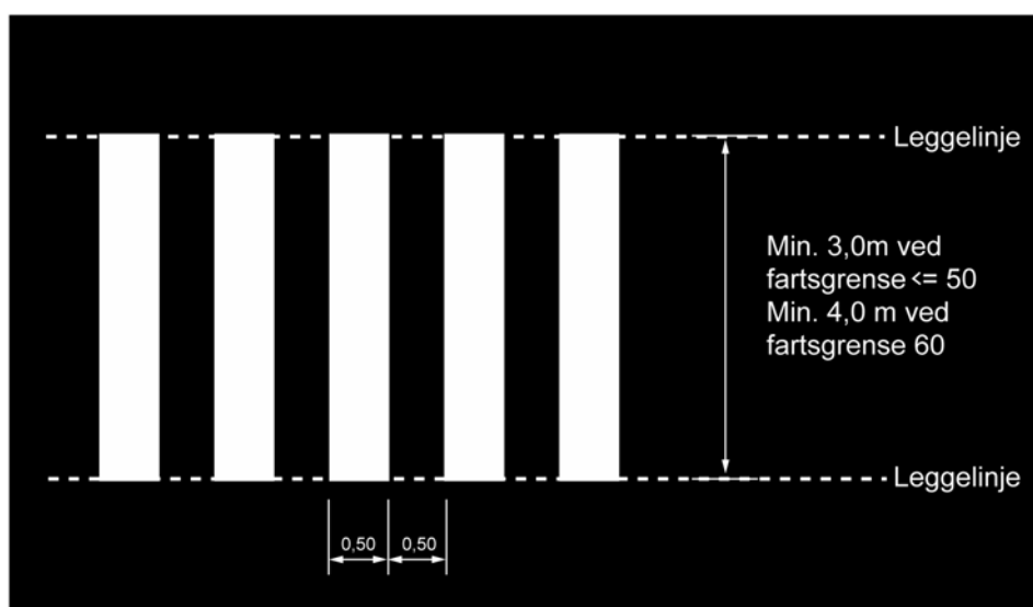
Figur 6.14: Skisse gangfelt
