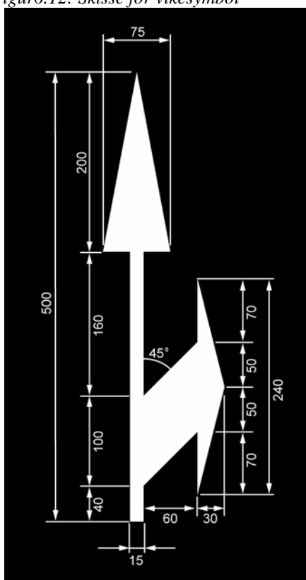
Figur 6.13: Skisse for piler
