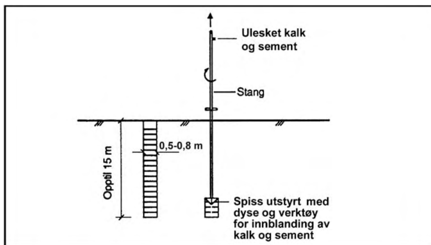
Figur 237.1 Kalk/sementpel – prinsipp tegning
