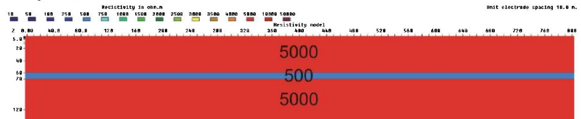
Figure 3.6.88: 10 m zone (500 ohmm) at a depth of 60m, V/H=1
