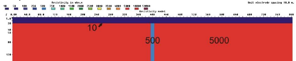
Figure 3.6.74: 10 m zone (500 ohmm) below a 20 m layer (10 ohmm), V/H=1
