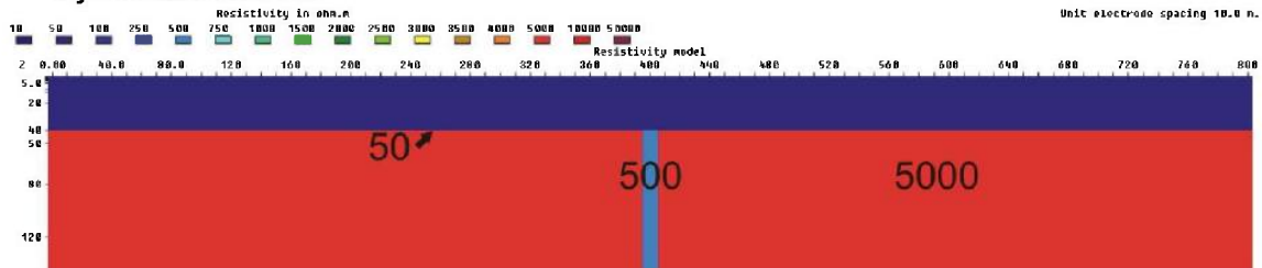
Figure 3.6.68: 10 m zone (500 ohmm) below a 40 m layer (50 ohmm), V/H=1
