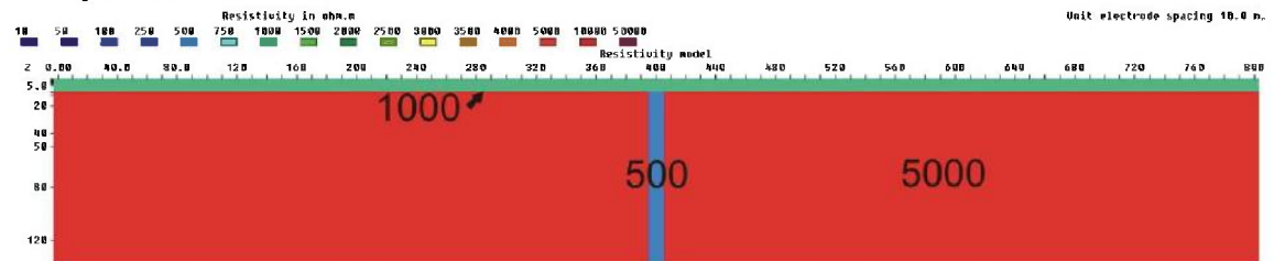
Figure 3.6.40: 10 m zone (500 ohmm) below a 10 m layer (1000 ohmm), V/H=1
