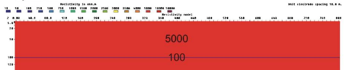
Figure 3.6.97: 1 m zone (100 ohmm) at a depth of 100m, V/H=0.5
