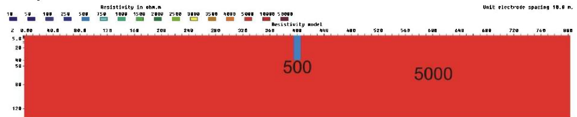
Figure 3.6.6: 10 m zone (500 ohmm) with a depth of 40 m, V/H=2
