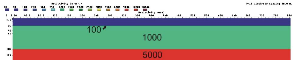
Figure 3.6.78: 3-layer model (100 ohmm, 1000 ohmm, 5000 ohmm), V/H=1
