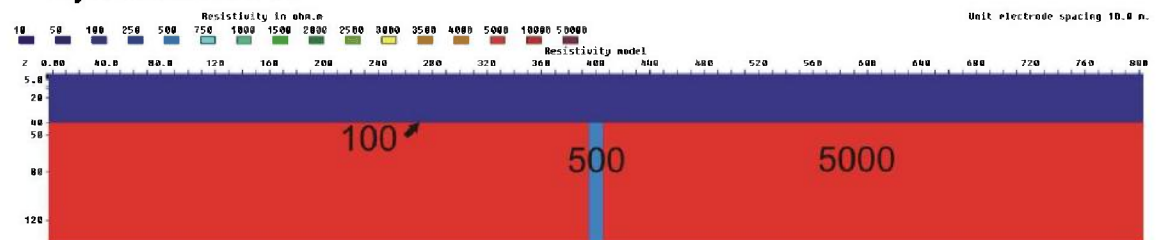
Figure 3.6.61: 10 m zone (500 ohmm) below a 40 m layer (100 ohmm), V/H=2
