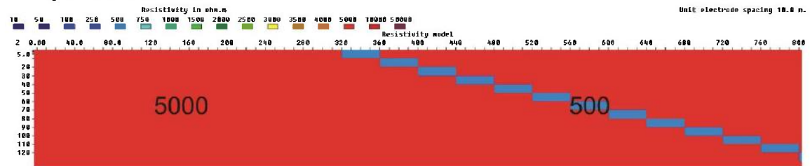
Figure 3.6.37: 10 m zone (500 ohmm) dipping with 15 degrees, V/H=0.5
