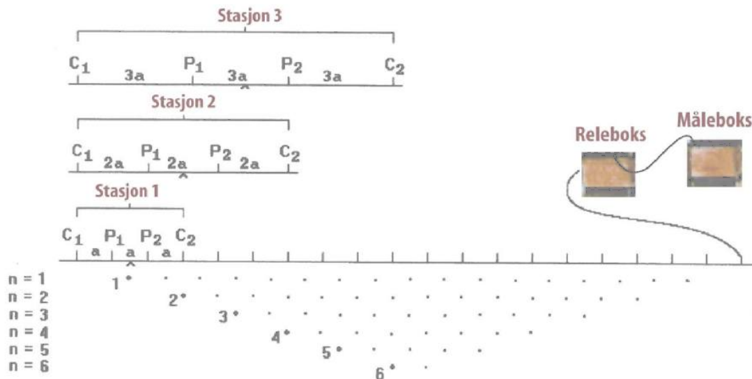
Figure 2.3: Roll along principle with the Wenner electrode configuration (After Barker 1992).
