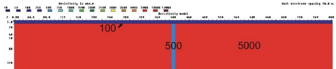
Figure 3.6.57: 10 m zone (500 ohmm) below a 10 m layer (100 ohmm), V/H=2
