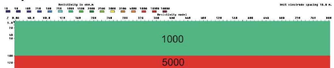
Figure 3.6.76: 2-layer model (1000 ohmm over 5000 ohmm), V/H=1
