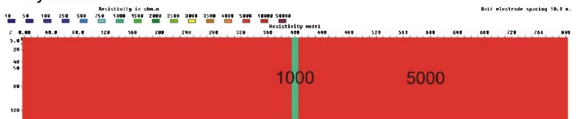
Figure 3.6.24: 10 m zone (1000 ohmm) in bedrock (5000 ohmm), V/H=2
