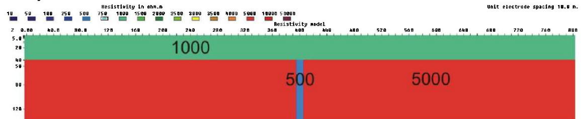
Figure 3.6.45: 10 m zone (500 ohmm) below a 40 m layer (1000 ohmm), V/H=2
