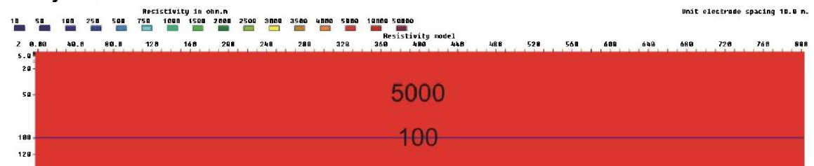
Figure 3.6.96: 1 m zone (100 ohm) at a depth of 100m, V/H=1
