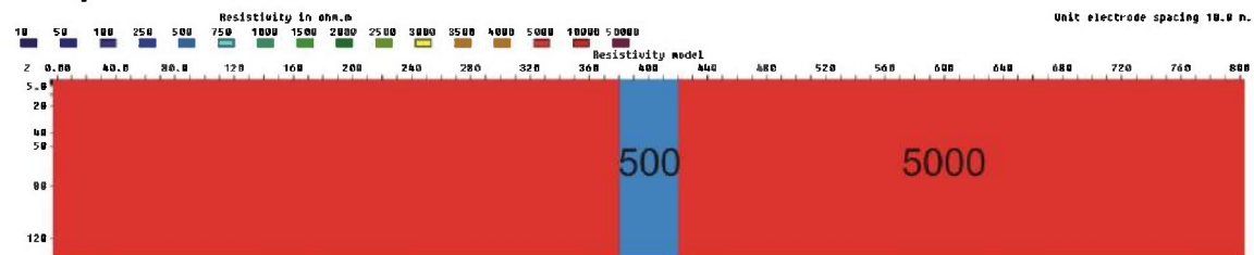
Figure 3.6.17: 40 m zone (500 ohmm), V/H=1
