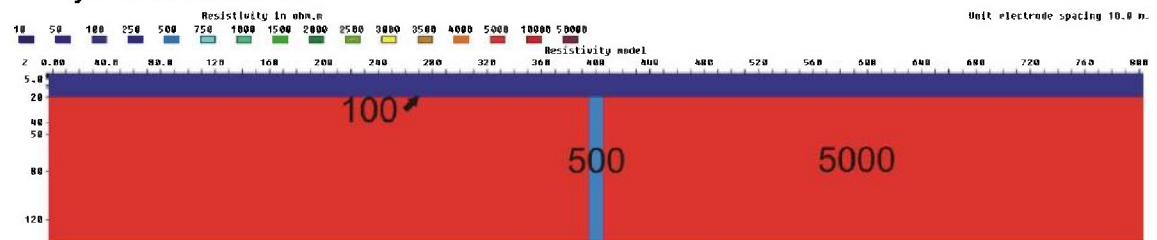
Figure 3.6.58: 10 m zone (500 ohmm) below a 20 m layer (100 ohmm), V/H=1
