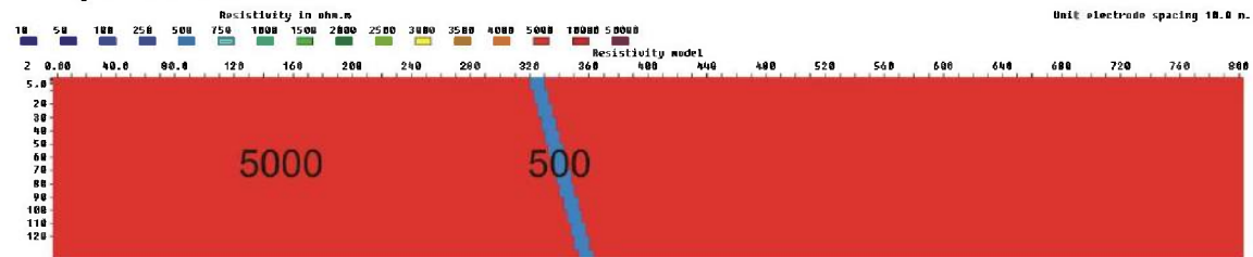
Figure 3.6.29: 10 m zone (500 ohmm) dipping with 75 degrees, V/H=1
