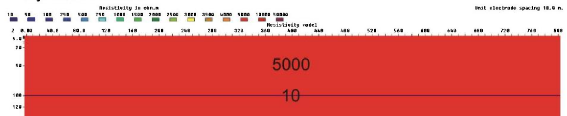
Figure 3.6.95: 1 m zone (10 ohmm) at a depth of 100m, V/H=0.5
