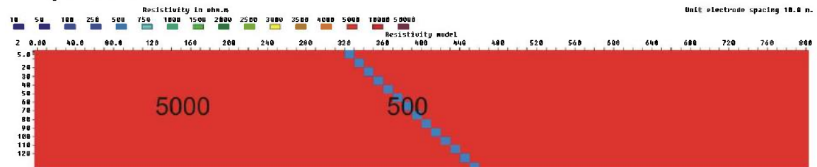
Figure 3.6.33: 10 m zone (500 ohmm) dipping with 45 degrees, V/H=1
