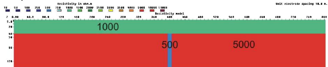
Figure 3.6.44: 10 m zone (500 ohmm) below a 40 m layer (1000 ohmm), V/H=1
