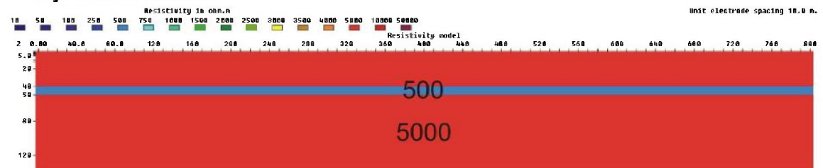
Figure 3.6.86: 10 m zone (500 ohmm) at a depth of 40m, V/H=1
