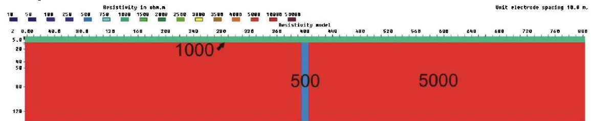
Figure 3.6.41: 10 m zone (500 ohmm) below a 10 m layer (1000 ohmm), V/H=2
