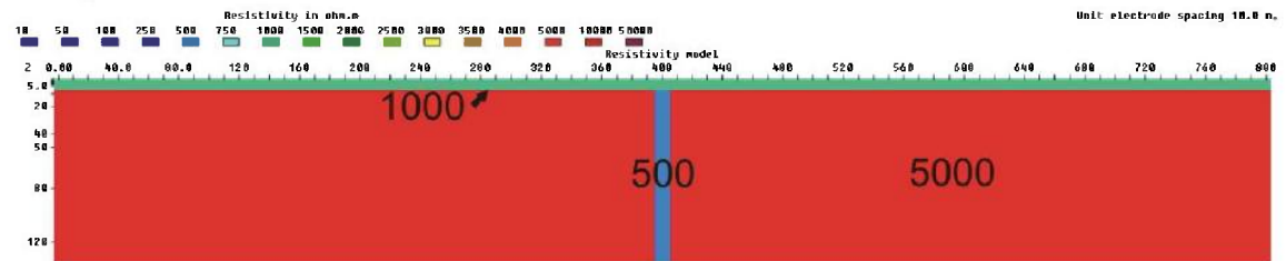
Figure 3.6.39: 10 m zone (500 ohmm) below a 5 m layer (1000 ohmm), V/H=2
