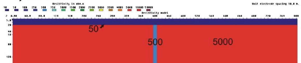
Figure 3.6.67: 10 m zone (500 ohmm) below a 20 m layer (50 ohmm), V/H=2
