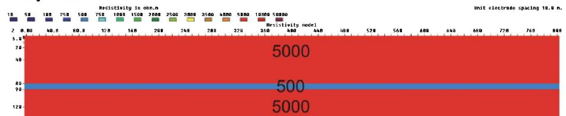
Figure 3.6.90: 10 m zone (500 ohmm) at a depth of 80m, V/H=1
