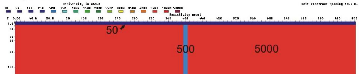
Figure 3.6.62: 10 m zone (500 ohmm) below a 5 m layer (50 ohmm), V/H=1
