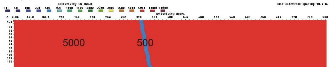
Figure 3.6.27: 10 m zone (500 ohmm) dipping with 80 degrees, V/H=1
