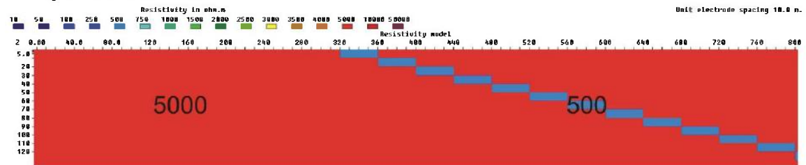
Figure 3.6.36: 10 m zone (500 ohmm) dipping with 15 degrees, V/H=1
