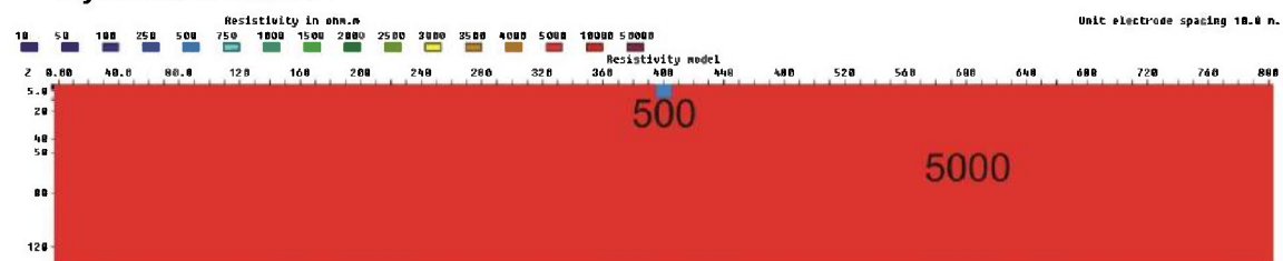
Figure 3.6.1: 10 m zone (500 ohmm) with a depth of 10 m, V/H=1
