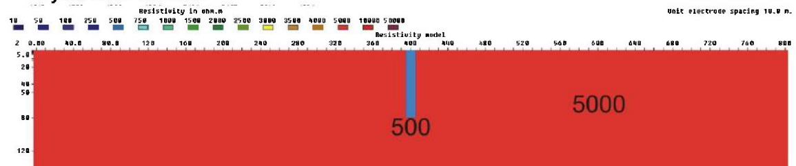
Figure 3.6.7: 10 m zone (500 ohmm) with a depth of 80 m, V/H=1
