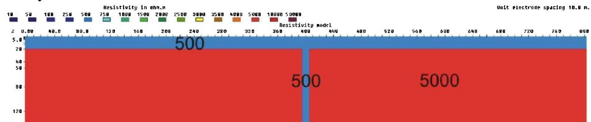
Figure 3.6.51: 10 m zone (500 ohmm) below a 20 m layer (500 ohmm), V/H=2
