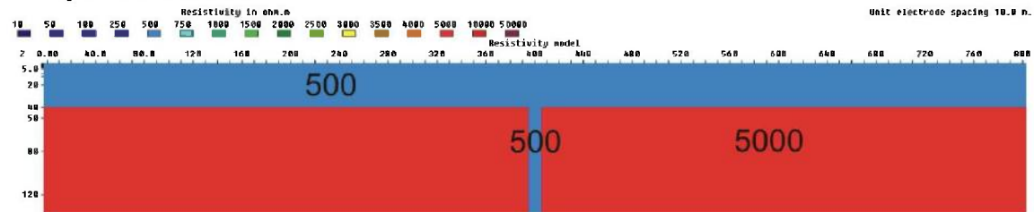
Figure 3.6.53: 10 m zone (500 ohm.m) below a 40 m layer (500 ohm.m), V/H=2
