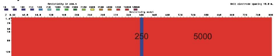
Figure 3.6.19: 10 m zone (250 ohmm) in bedrock (5000 ohmm), V/H=1
