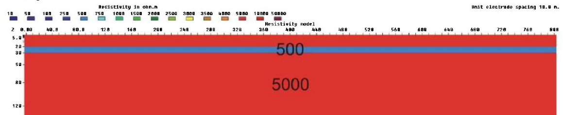
Figure 3.6.85: 10 m zone (500 ohmm) at a depth of 20m, V/H=0.5
