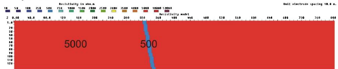
Figure 3.6.28: 10 m zone (500 ohmm) dipping with 80 degrees, V/H=2
