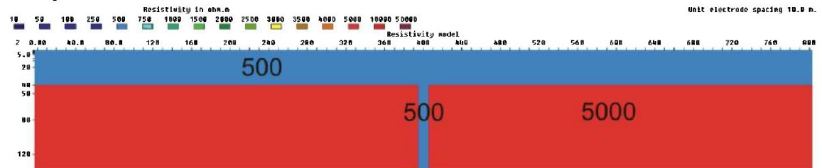
Figure 3.6.52: 10 m zone (500 ohmm) below a 40 m layer (500 ohmm), V/H=1
