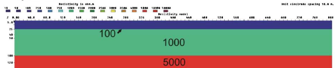
Figure 3.6.79: 3-layer model (100 ohmm, 1000 ohmm, 5000 ohmm), V/H=0.5
