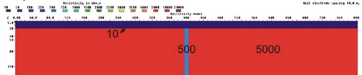
Figure 3.6.75: 10 m zone (500 ohmm) below a 20 m layer (10 ohmm), V/H=2
