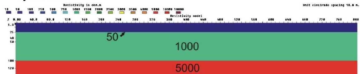
Figure 3.6.80: 3-layer model (50 ohmm, 1000 ohmm, 5000 ohmm), V/H=1
