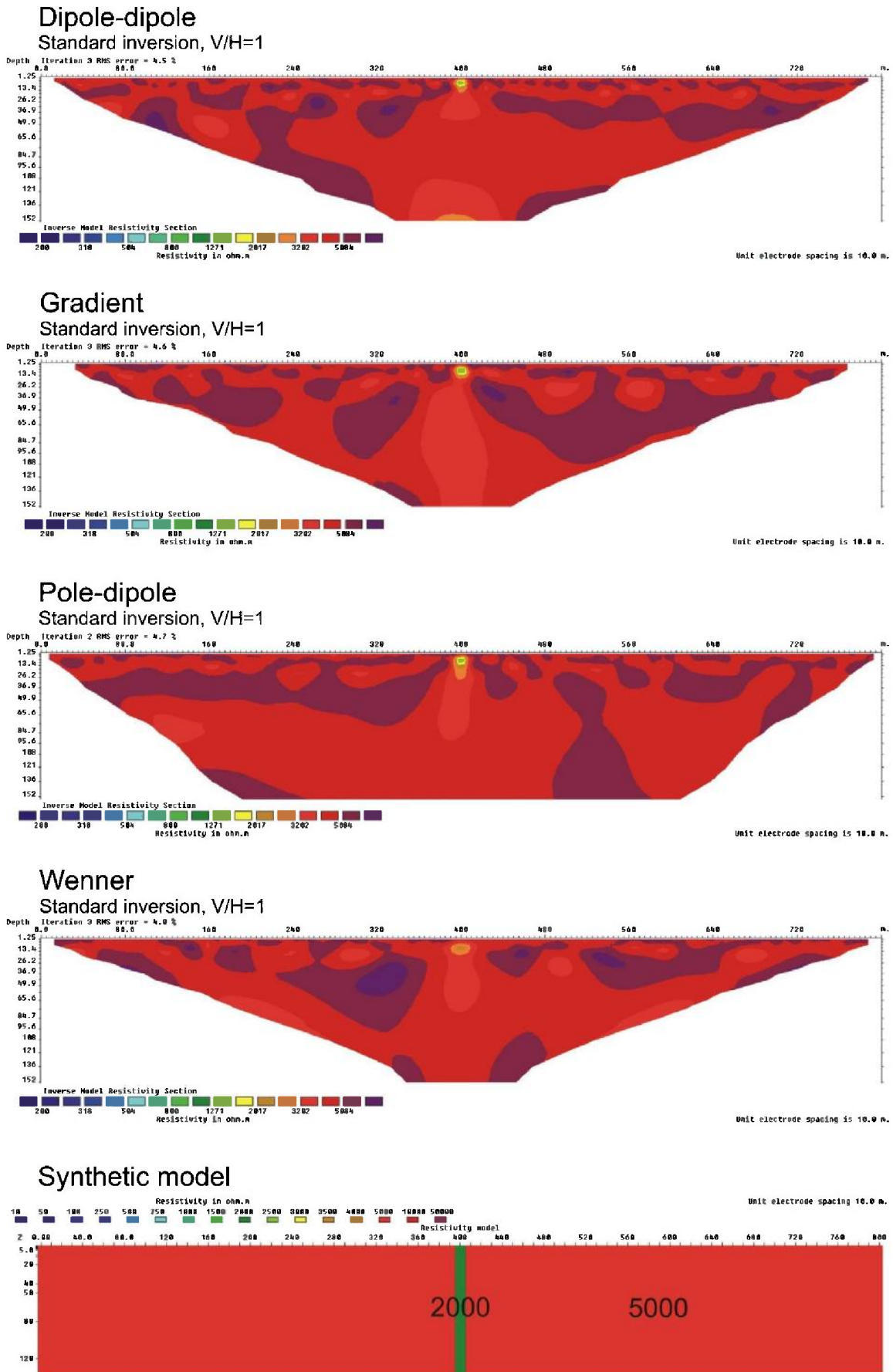
Figure 3.6.25: 10 m zone (2000 ohm) in bedrock (5000 ohm), V/H=1
