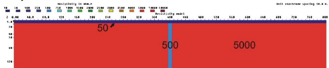
Figure 3.6.63: 10 m zone (500 ohmm) below a 5 m layer (50 ohmm), V/H=2
