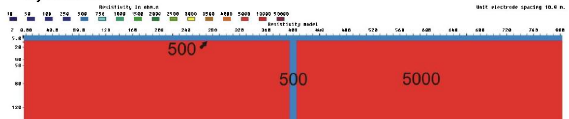
Figure 3.6.46: 10 m zone (500 ohmm) below a 5 m layer (500 ohmm), V/H=1
