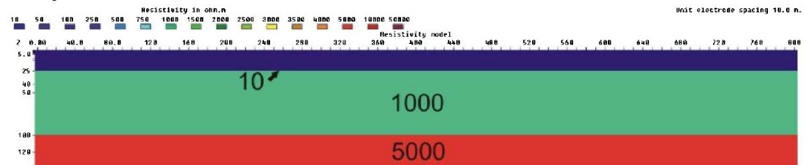
Figure 3.6.83: 3-layer model (10 ohmm, 1000 ohmm, 5000 ohmm), V/H=0.5
