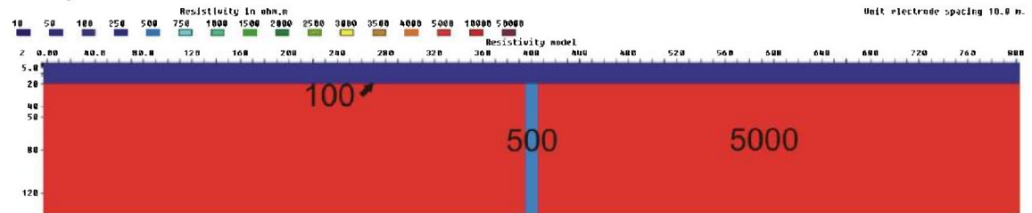
Figure 3.6.59: 10 m zone (500 ohmm) below a 20 m layer (100 ohmm), V/H=2
