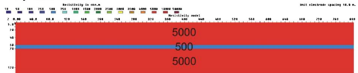
Figure 3.6.89: 10 m zone (500 ohmm) at a depth of 60m, V/H=0.5
