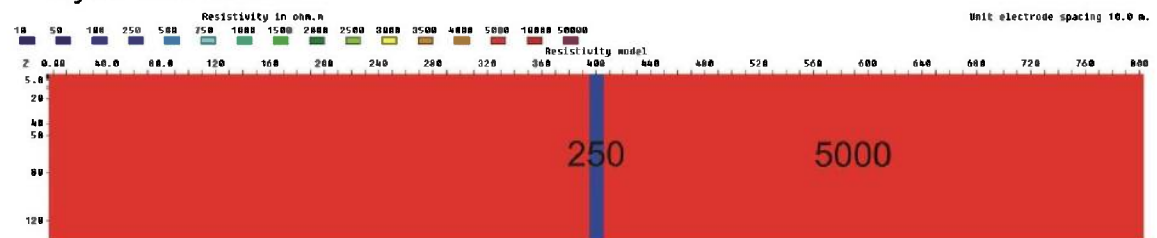
Figure 3.6.20: 10 m zone (250 ohmm) in bedrock (5000 ohmm), V/H=2
