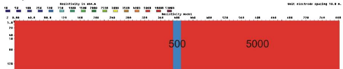
Figure 3.6.16: 20 m zone (500 ohmm), V/H=2
