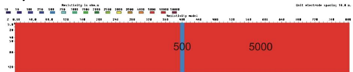
Figure 3.6.22: 10 m zone (500 ohmm) in bedrock (5000 ohmm), V/H=2
