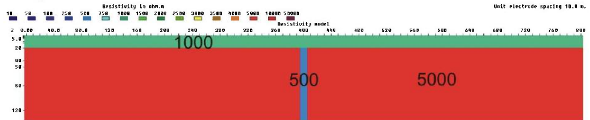
Figure 3.6.43: 10 m zone (500 ohmm) below a 20 m layer (1000 ohmm), V/H=2
