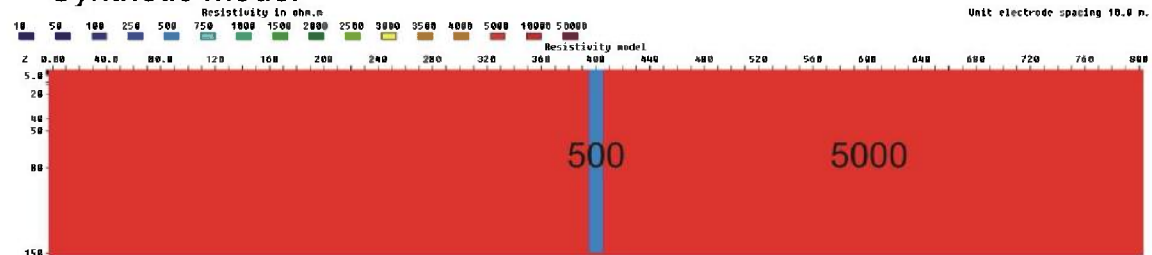
Figure 3.6.9: 10 m zone (500 ohmm) with a depth of 150 m, V/H=1
