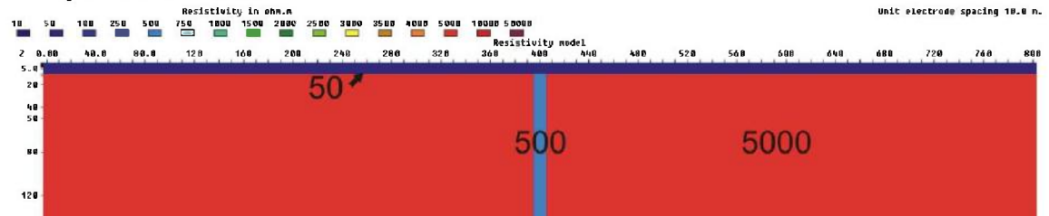
Figure 3.6.65: 10 m zone (500 ohmm) below a 10 m layer (50 ohmm), V/H=2
