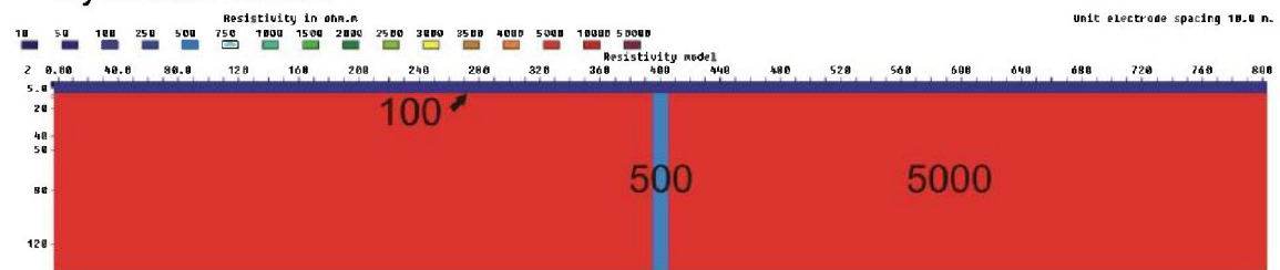
Figure 3.6.55: 10 m zone (500 ohmm) below a 5 m layer (100 ohmm), V/H=2
