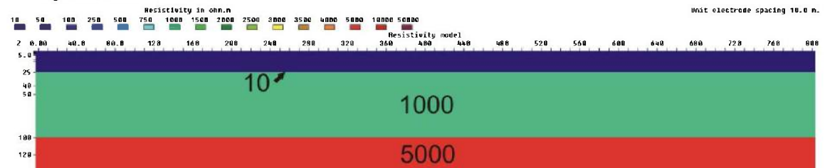
Figure 3.6.82: 3-layer model (10 ohmm, 1000 ohmm, 5000 ohmm), V/H=1
