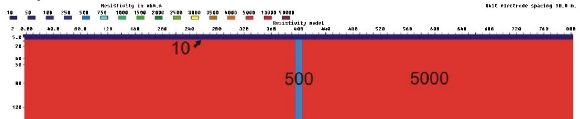
Figure 3.6.71: 10 m zone (500 ohmm) below a 5 m layer (10 ohmm), V/H=2
