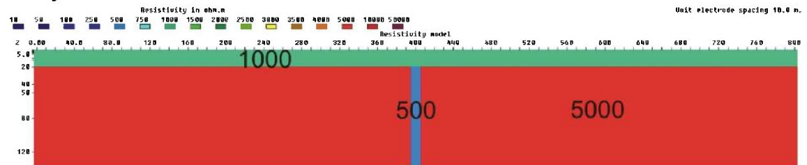
Figure 3.6.42: 10 m zone (500 ohmm) below a 20 m layer (1000 ohmm), V/H=1
