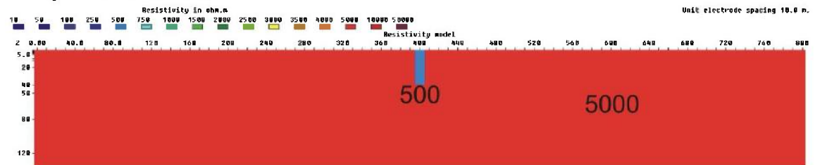
Figure 3.6.5: 10 m zone (500 ohmm) with a depth of 40 m, V/H=1
