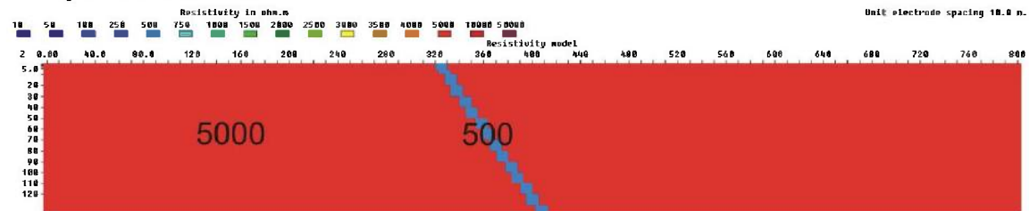
Figure 3.6.32: 10 m zone (500 ohmm) dipping with 60 degrees, V/H=2
