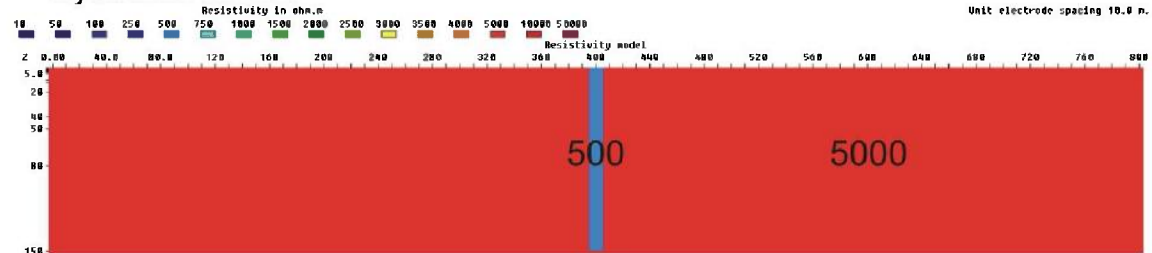
Figure 3.6.10: 10 m zone (500 ohmm) with a depth of 150 m, V/H=2
