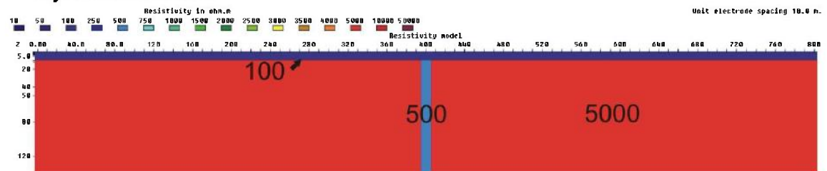
Figure 3.6.56: 10 m zone (500 ohmm) below a 10 m layer (100 ohmm), V/H=1
