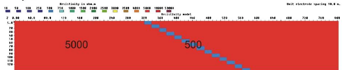
Figure 3.6.34: 10 m zone (500 ohmm) dipping with 30 degrees, V/H=1
