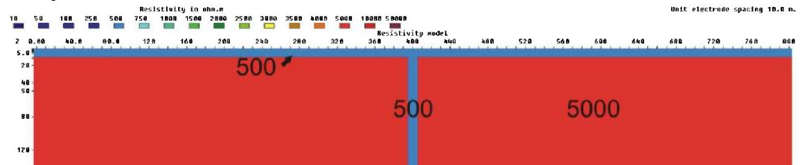
Figure 3.6.49: 10 m zone (500 ohmm) below a 10 m layer (500 ohmm), V/H=2
