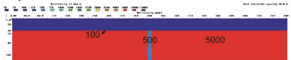
Figure 3.6.60: 10 m zone (500 ohmm) below a 40 m layer (100 ohmm), V/H=1
