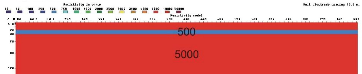
Figure 3.6.84: 10 m zone (500 ohmm) at a depth of 20m, V/H=1
