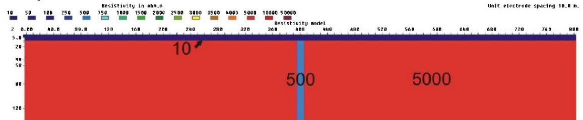
Figure 3.6.72: 10 m zone (500 ohmm) below a 10 m layer (10 ohmm), V/H=1
