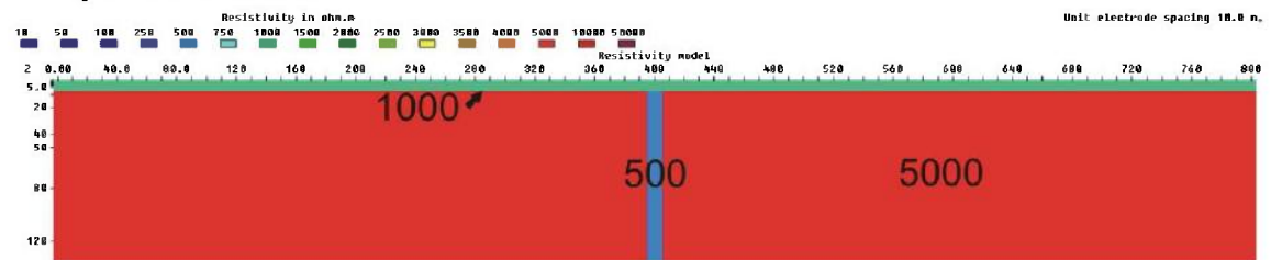
Figure 3.6.38: 10 m zone (500 ohmm) below a 5 m layer (1000 ohmm), V/H=1
