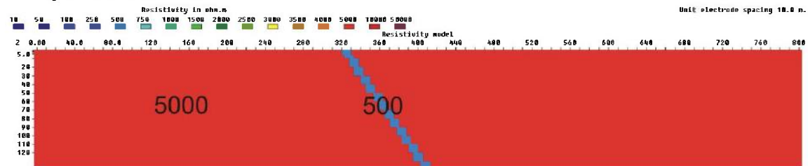
Figure 3.6.31: 10 m zone (500 ohmm) dipping with 60 degrees, V/H=1
