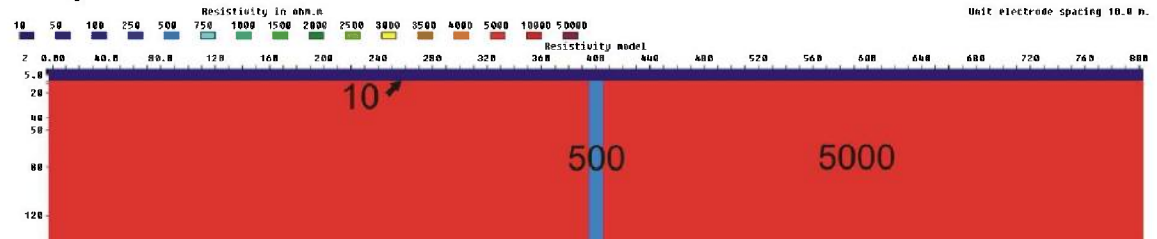
Figure 3.6.73: 10 m zone (500 ohmm) below a 10 m layer (10 ohmm), V/H=2
