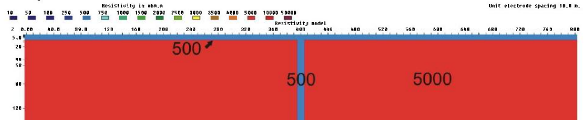
Figure 3.6.47: 10 m zone (500 ohmm) below a 5 m layer (500 ohmm), V/H=2
