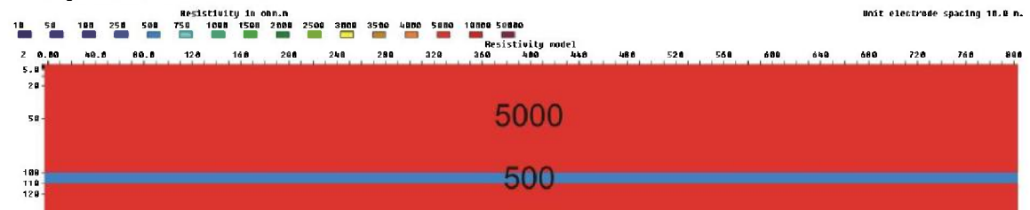
Figure 3.6.92: 10 m zone (500 ohmm) at a depth of 100m, V/H=1
