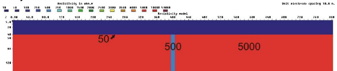
Figure 3.6.69: 10 m zone (500 ohmm) below a 40 m layer (50 ohmm), V/H=2
