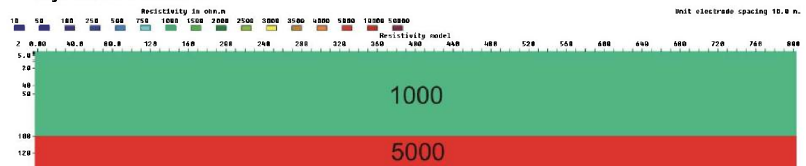
Figure 3.6.77: 2-layer model (1000 ohmm over 5000 ohmm), V/H=0.5
