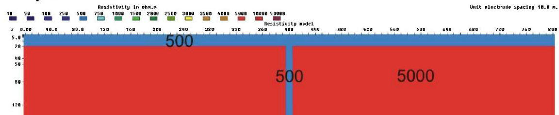
Figure 3.6.50: 10 m zone (500 ohmm) below a 20 m layer (500 ohmm), V/H=1
