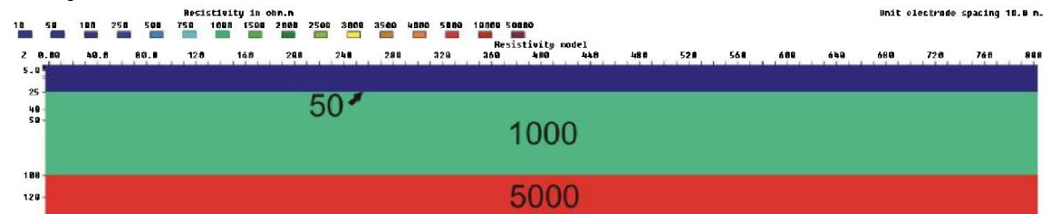
Figure 3.6.81: 3-layer model (50 ohmm, 1000 ohmm, 5000 ohmm), V/H=0.5
