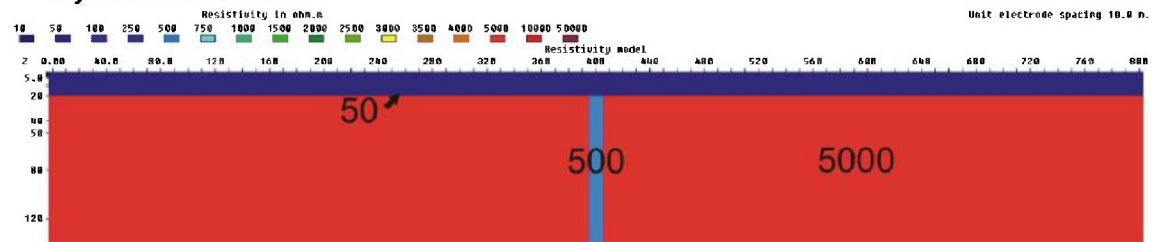
Figure 3.6.66: 10 m zone (500 ohmm) below a 20 m layer (50 ohmm), V/H=1
