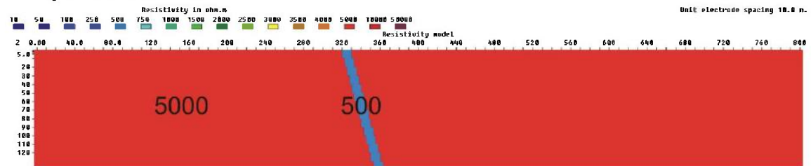
Figure 3.6.30: 10 m zone (500 ohmm) dipping with 75 degrees, V/H=2
