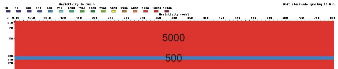
Figure 3.6.93: 10 m zone (500 ohmm) at a depth of 100m, V/H=0.5
