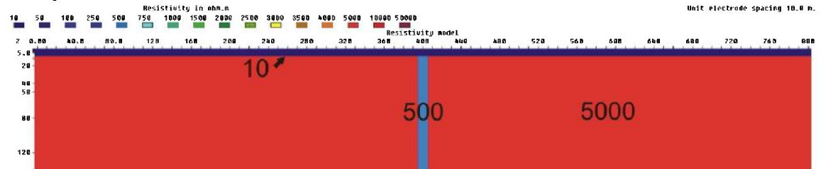
Figure 3.6.70: 10 m zone (500 ohmm) below a 5 m layer (10 ohmm), V/H=1
