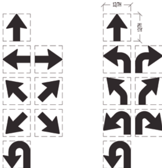
Figur 4-4.3 Standard piler for tabellskilt
