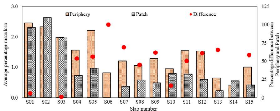
Fig. 15. Average percentage mass loss of the steel bars in the "patch" and the peripheral region for the different slabs.
