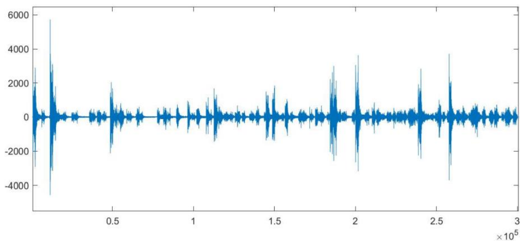
Figure 37 Vertical acceleration recorded on the H18_E accelerometer during a 100 minutes long interval. The x-axis gives a sample number and the y-axis acceleration in \mu g
