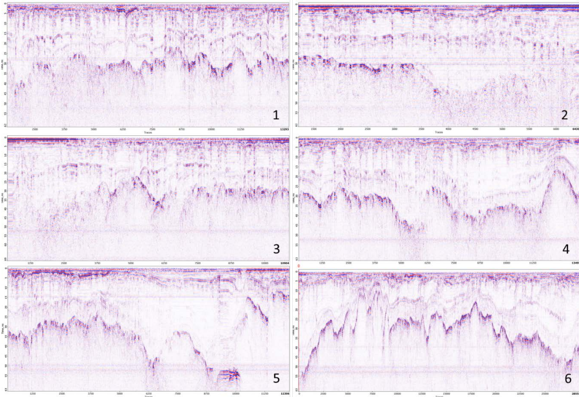
Figure 3-7. Ground (sled) GPR profiles. The profile numbers (1 to 6) correspond to surveys plotted in Figure 3-6. The end of profile 2 corresponds to snow pit B-2 and the end of profile 6 corresponds to snow pit B-1. Calibration of GPR data with ground truth from the snow pit will be completed, at least for the shallow layers.
