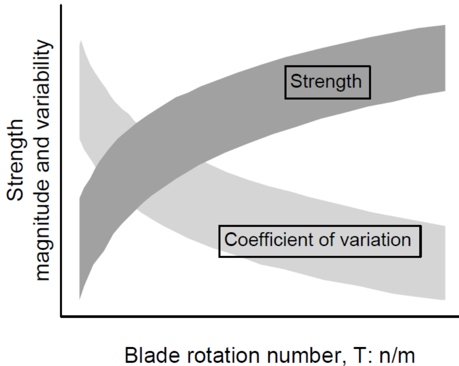
Figure 3.1. Effect of blade rotation number on the strength and variability of the stabilised soil (Larsson 2005).
