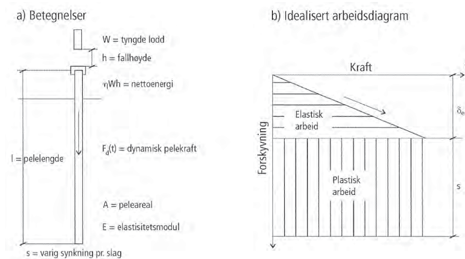
Figur 11.11 Rammeformel - prinsippsskisser.
