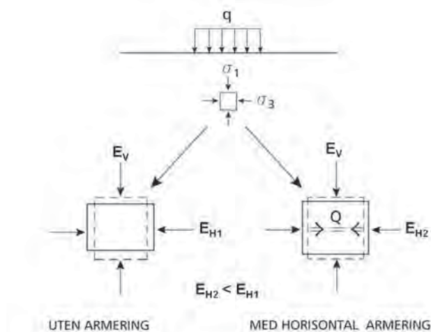
Figur 16.3 Jordarmering -prinsipp. (Etter; Carlsson 1989, Ref. 11)
