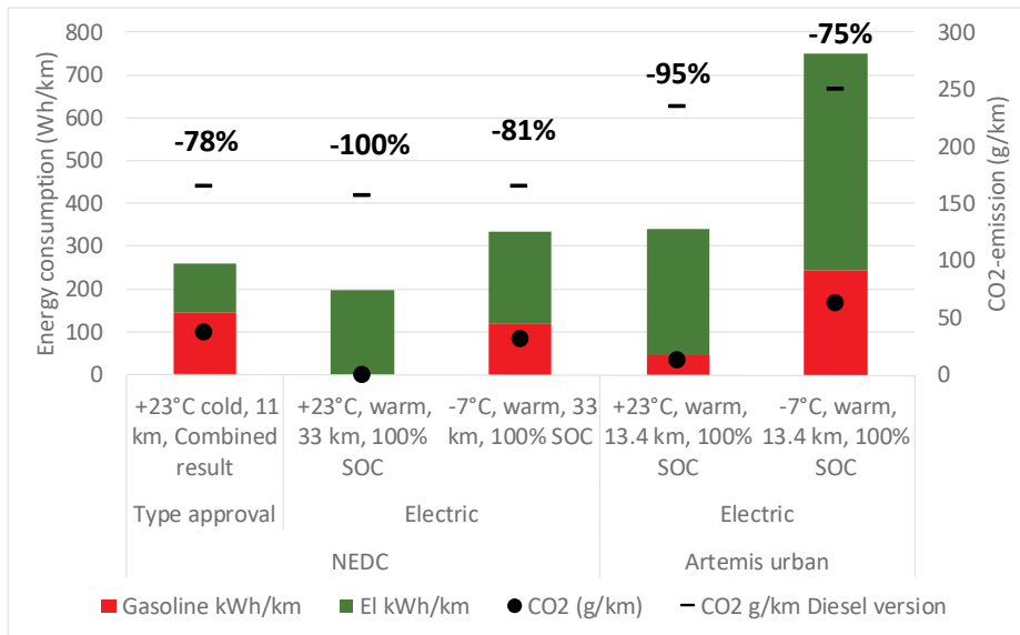
Figure 3.1: Vehicle A, measured E-mode energy consumption (Wh/km) and CO 2 -emission (g/km), compared to official type approval values, and EMIROAD measured CO 2 -emission of a comparable diesel vehicle (g/km). CO 2 -emission reduction versus diesel version is also shown (percentage).
