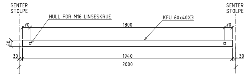
STANDARDPANEL PLAN 1:10
