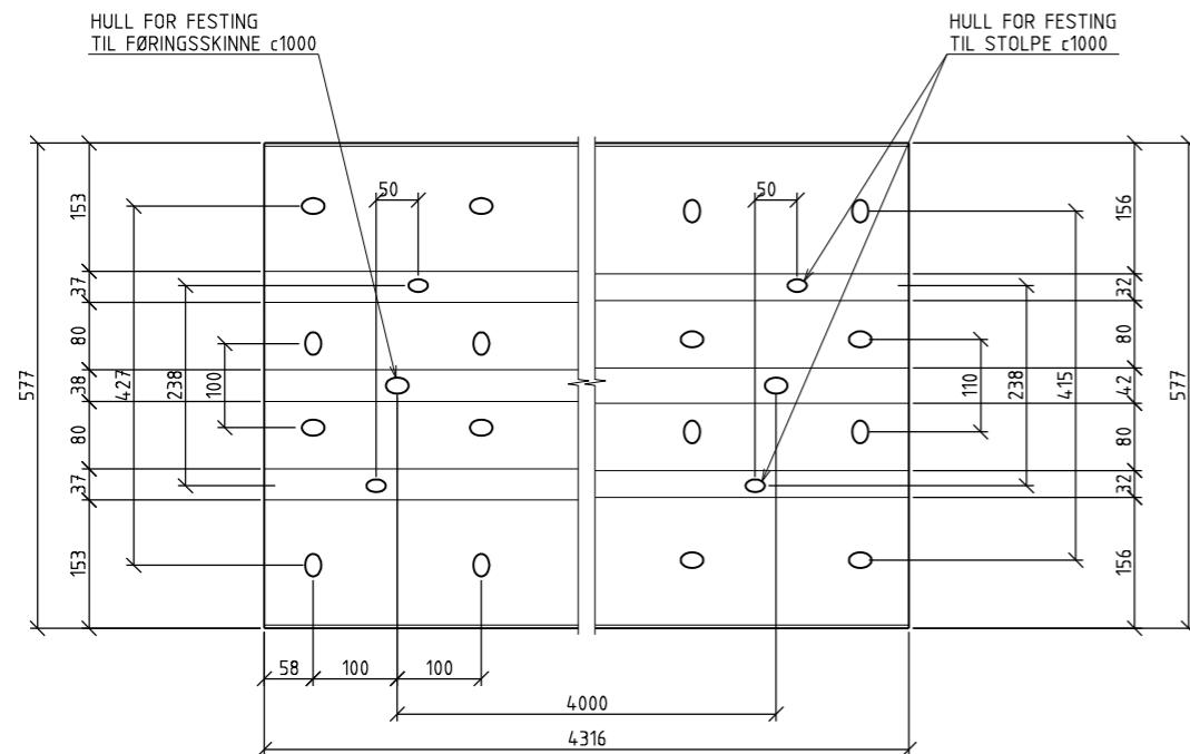
STANDARD BAKSKINNE UTFOLDET 1:5
