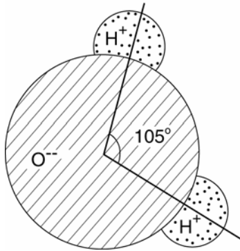
Figur 14.1 Vannmolekylet
