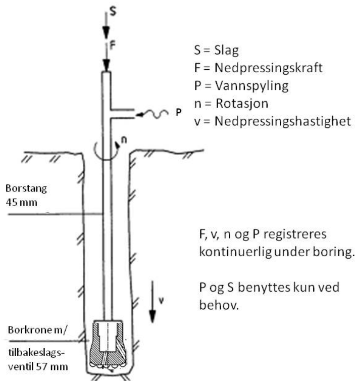
Figur 1.12 Totalsondering - prinsipp.
