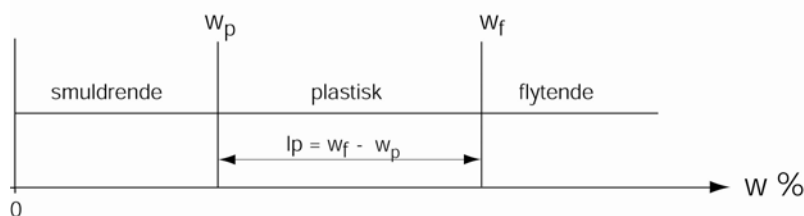
Figur 2.5 Konsistensgrensene
