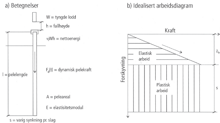
Figur 11. 11 Rammeformel - prinsippsskisser.
