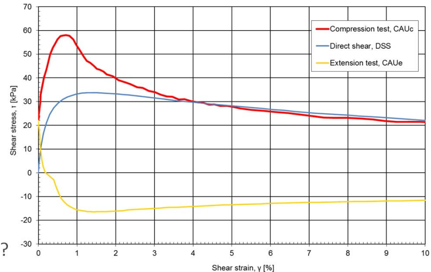
Parallel CAUC/ DSS/ CAUE tests on block sample E6 Øst - borehole 823, 9.2 m depth
